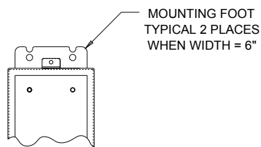
MOUNTING FOOT DETAIL
