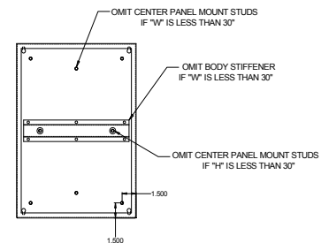
VIEW WITH COVER REMOVED
